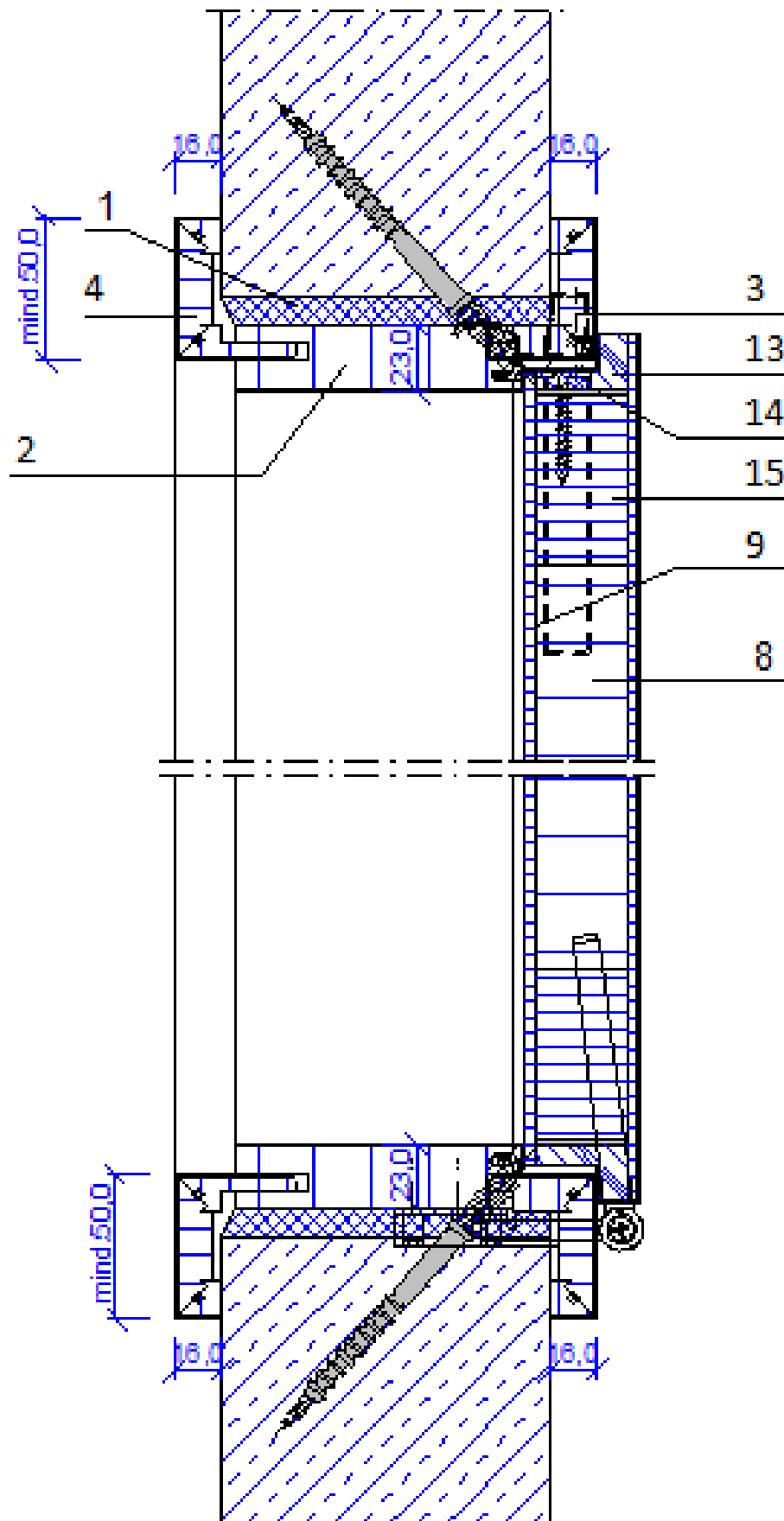
Figure 4 – Coupe horizontale – Type B
