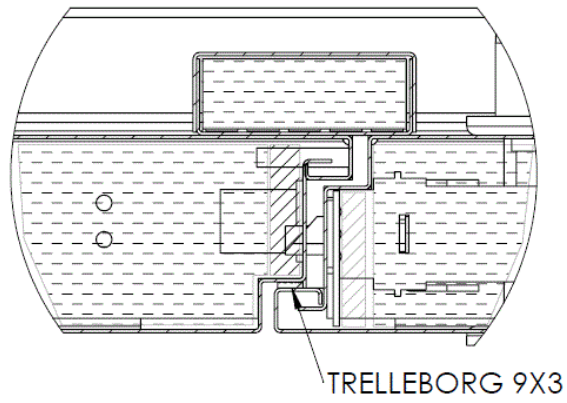
Fig. 7: Detail beglazing
